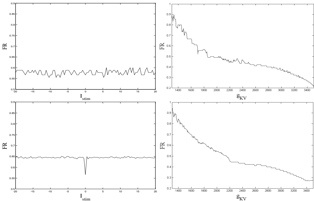
Figure 9. Changes of FR in various parts of neurons with parameters. (Top left): FR - I_{stim} diagram of the soma; (Top right): FR - g_{KV} diagram of the soma; (Bottom left): FR - I_{stim} diagram of the terminal button of the central axon; (Bottom right): FR - g_{KV} diagram of the terminal button of the central axon
