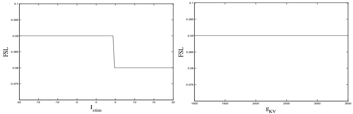
Figure 8. (Left): Changes of FSL with I_{stim} . (Right): Changes of FSL with g_{KV}
