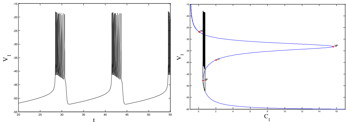
Figure 3. The “fold/homoclinic” bursting via the “fold/homoclinic” hysteresis loop in the system (4)~(9) when g_{KV} = 1350 \text{ s}^{-1}, V_K = -75 \text{ mV} . (Left): Time series of the membrane potential; (Right): Fast-slow dynamics bifurcation diagram
