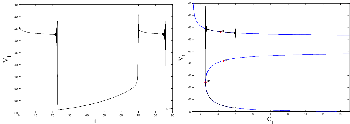
Figure 4. The “Hopf/homoclinic” bursting via the “fold/homoclinic” hysteresis loop in the system (4)~(9) when g_{KV} = 1000 \text{ s}^{-1}, V_K = -75 \text{ mV} . (Left): Time series of the membrane potential; (Right): Fast-slow dynamics bifurcation diagram
