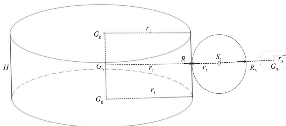
Figure 6. Schematic diagram of the gravitational effect of the galaxy 2 图 6. 星系引力作用示意图 2
