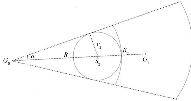
Figure 5. Schematic diagram of residual mass equivalence of galaxies
