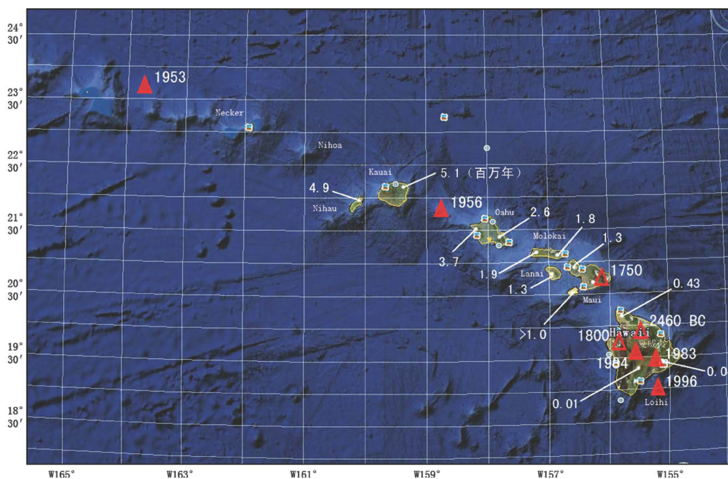
Figure 8. Rise and fall of the volcanoes in Hawaii islands (Base map from Google Earth 2013)
