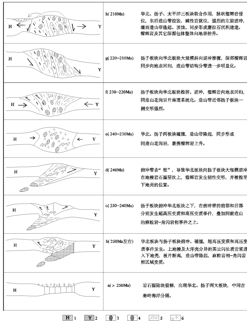
Figure 3. Collision and exhumation model of Dabie-Sulu orogenic belt; 1: North China Craton; 2: South China Craton; 3: ultrahigh-pressure rock; 4: high-pressure rock; 5: ductile shear zone; 6: surface crust
