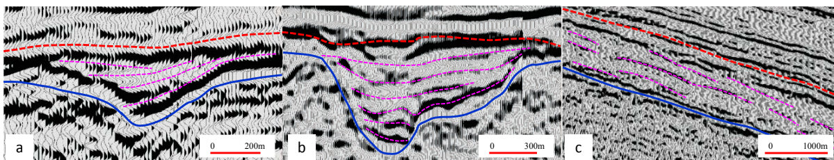
Figure 3. Seismic reflection characteristics of incised valley (according to ref. [25]) 图 3. 下切谷地震剖面反射特征(据文献[25])
