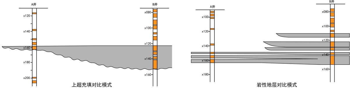
Figure 5. Stratigraphic comparison model (modified from ref. [37])
