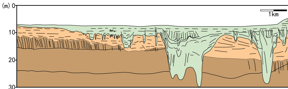
Figure 2. Geometry diagram of incised valley 图 2. 下切谷几何形态示意图
