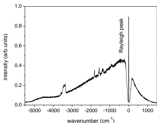
Figure 4. The Raman shift of blending oil 图 4. 调和油的拉曼频移图
