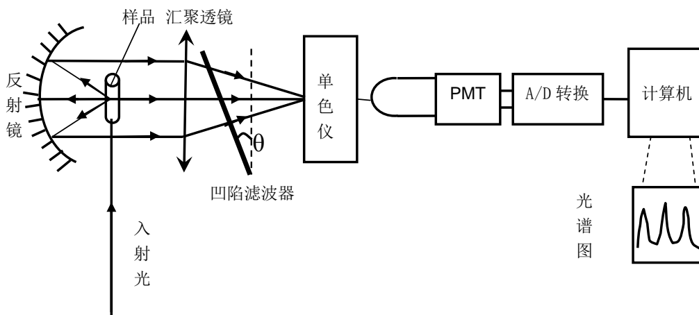
Figure 1. Schematic diagram of experiments 图 1. 实验原理图
