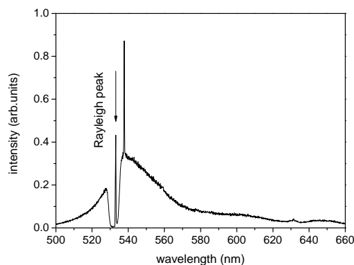
Figure 3. The Raman spectrum of gel water 图3. 啫喱水的拉曼光谱图
