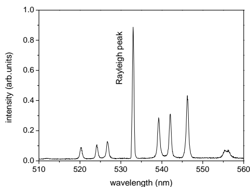
Figure 2. The Raman spectrum of carbon tetrachloride 图2. \text{CCl}_4 的拉曼光谱图
