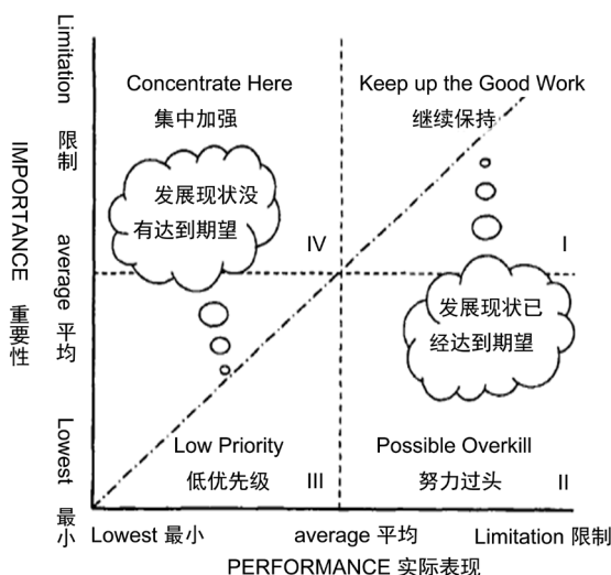
Figure 1. IPA positioning analysis diagram
