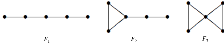
Figure 1. The avoiding induced subgraphs 图 1. G 的导出子图的禁图
