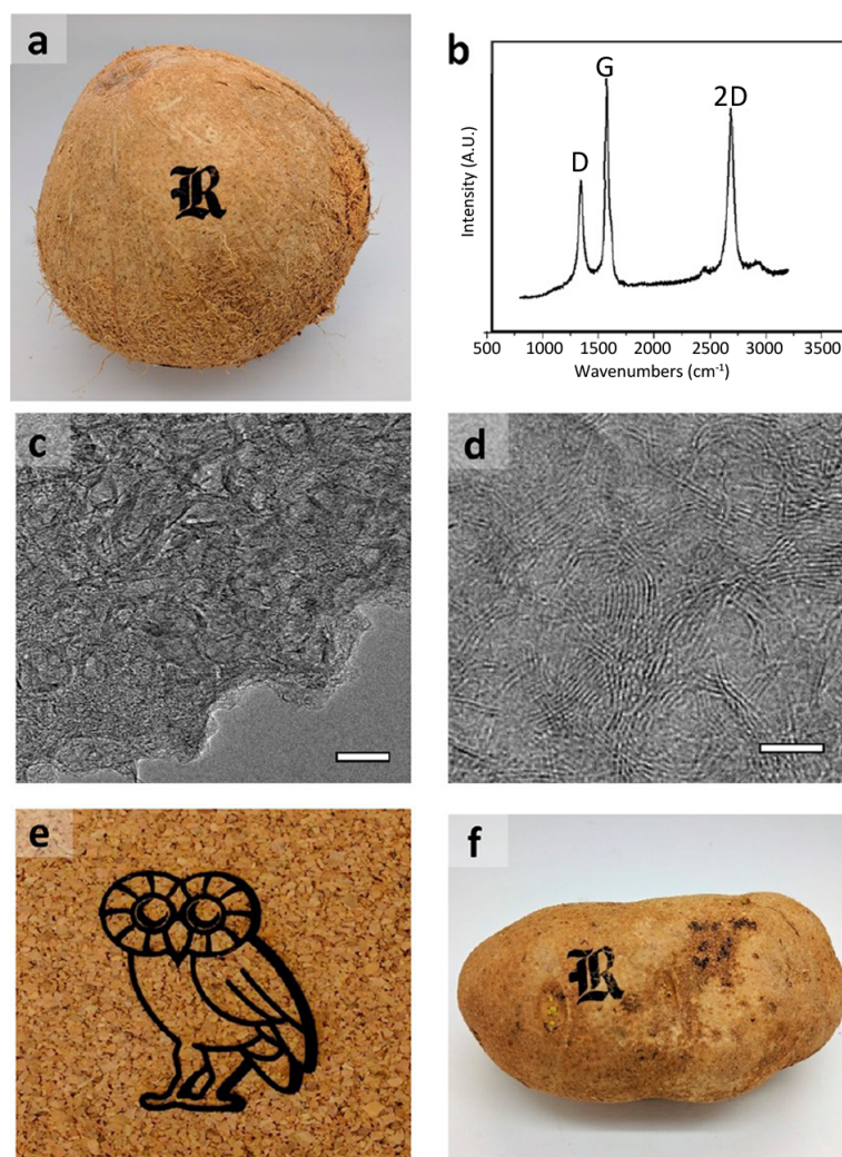
Figure 2. Preparation and characterization of graphene on coconut, bread and potato skins
