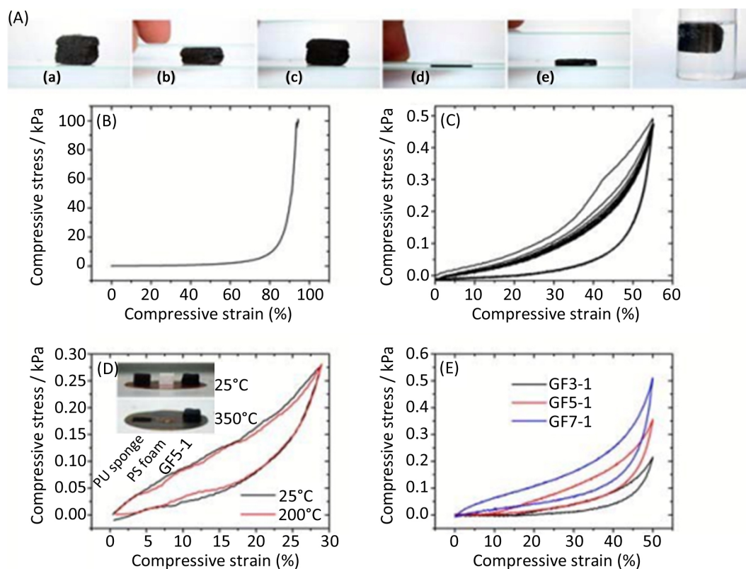
Figure 3. Mechanical properties of three-dimensional graphene foam
