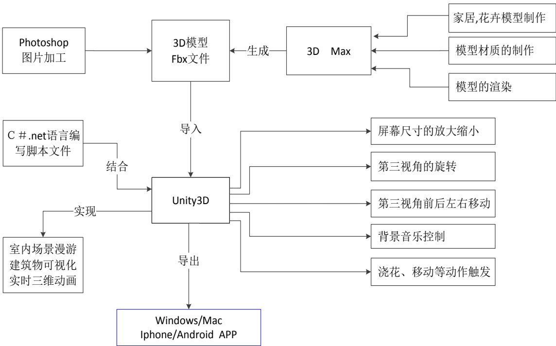
Figure 3. Schematic diagram of client application development process 图 3. 客户端应用程序开发流程示意图
