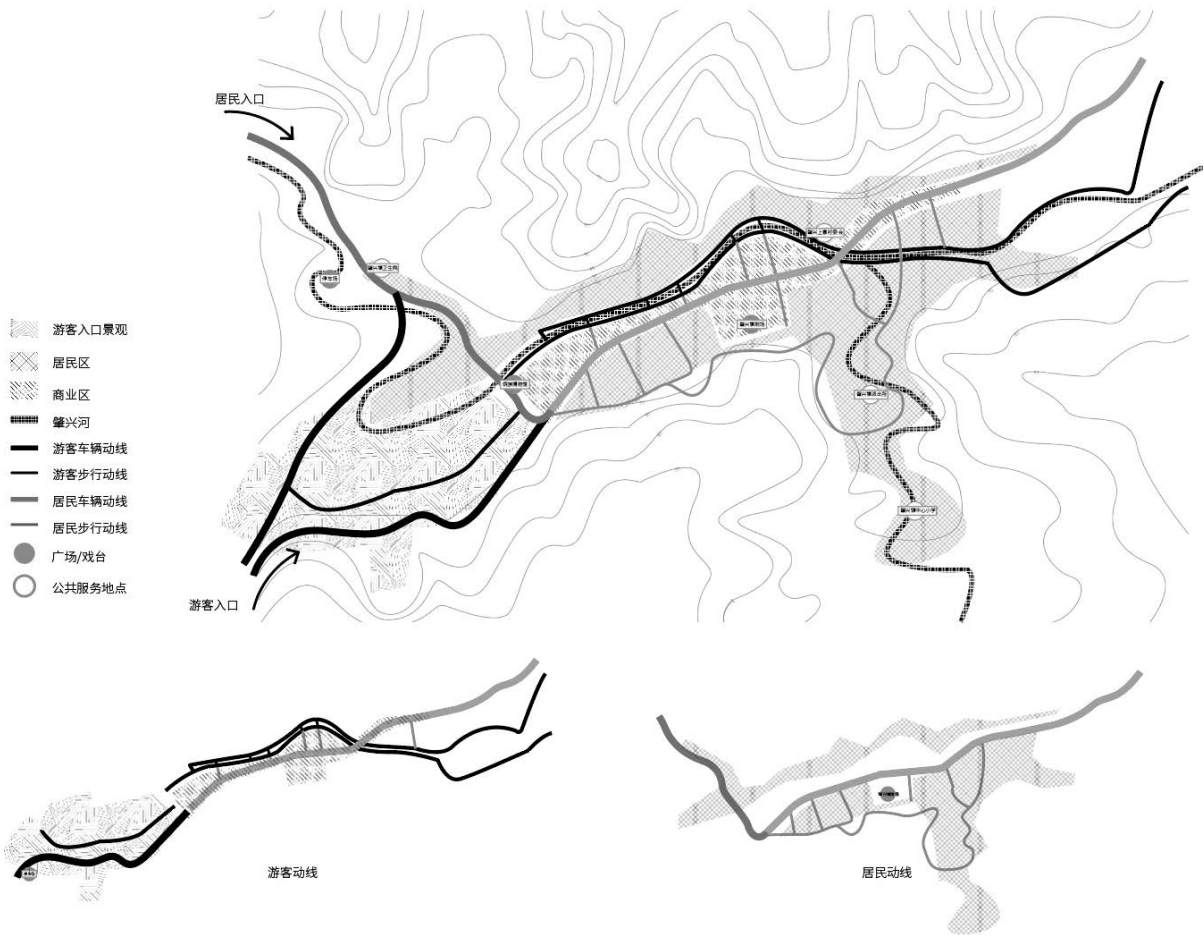
Figure 13. Zhaoxing Town main traffic route map and diversion plan for residents and tourists 图 13. 肇兴镇主动线图及居民游客分流方案 ⑭
