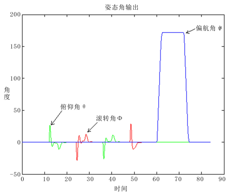
Figure 5. The response line of attitude angle
