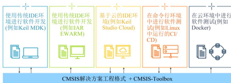
Figure 8. An open workflow involving CMSIS-Toolbox
