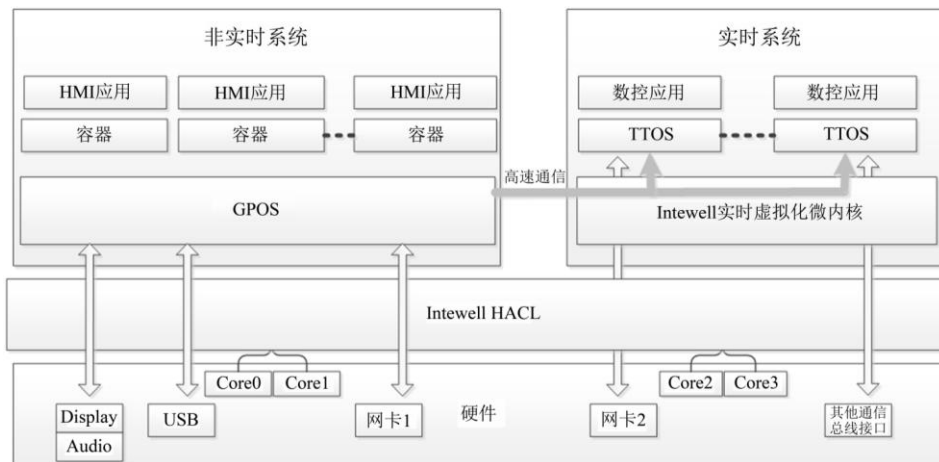
Figure 4. Intewell configurable hybrid heterogeneous system architecture
