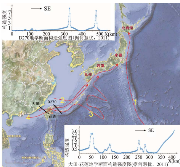
Figure 9. Geosciences' transect location and structural strength map of Datian-Hualian and D270
