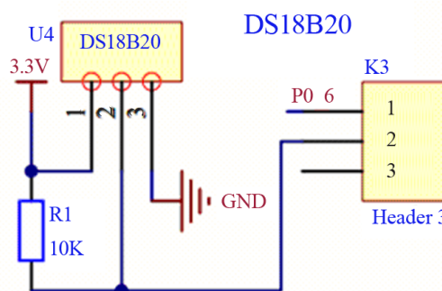
Figure 3. Circuit Diagram of Temperature Sensor 图 3. 温度传感器电路图
