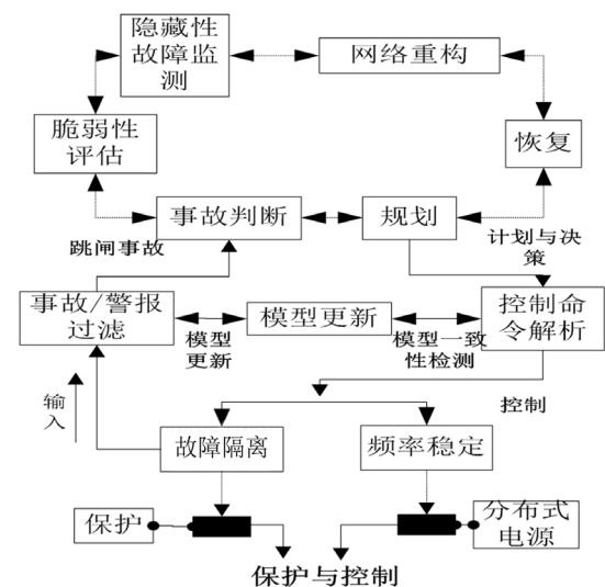
Figure 2. System layer structure of SPID 图 2. SPID 监控层结构
