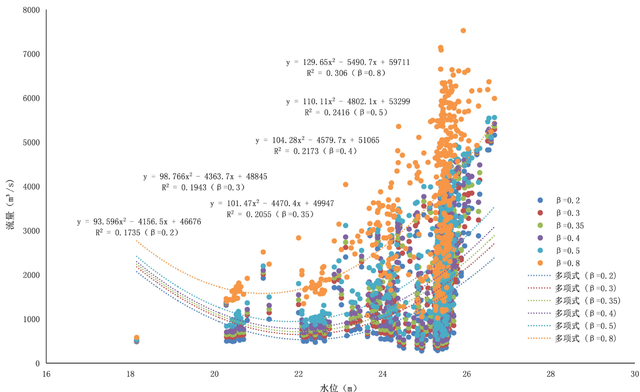
Figure 2. Correlation analysis diagram of flow with drop less than 0.7 m
