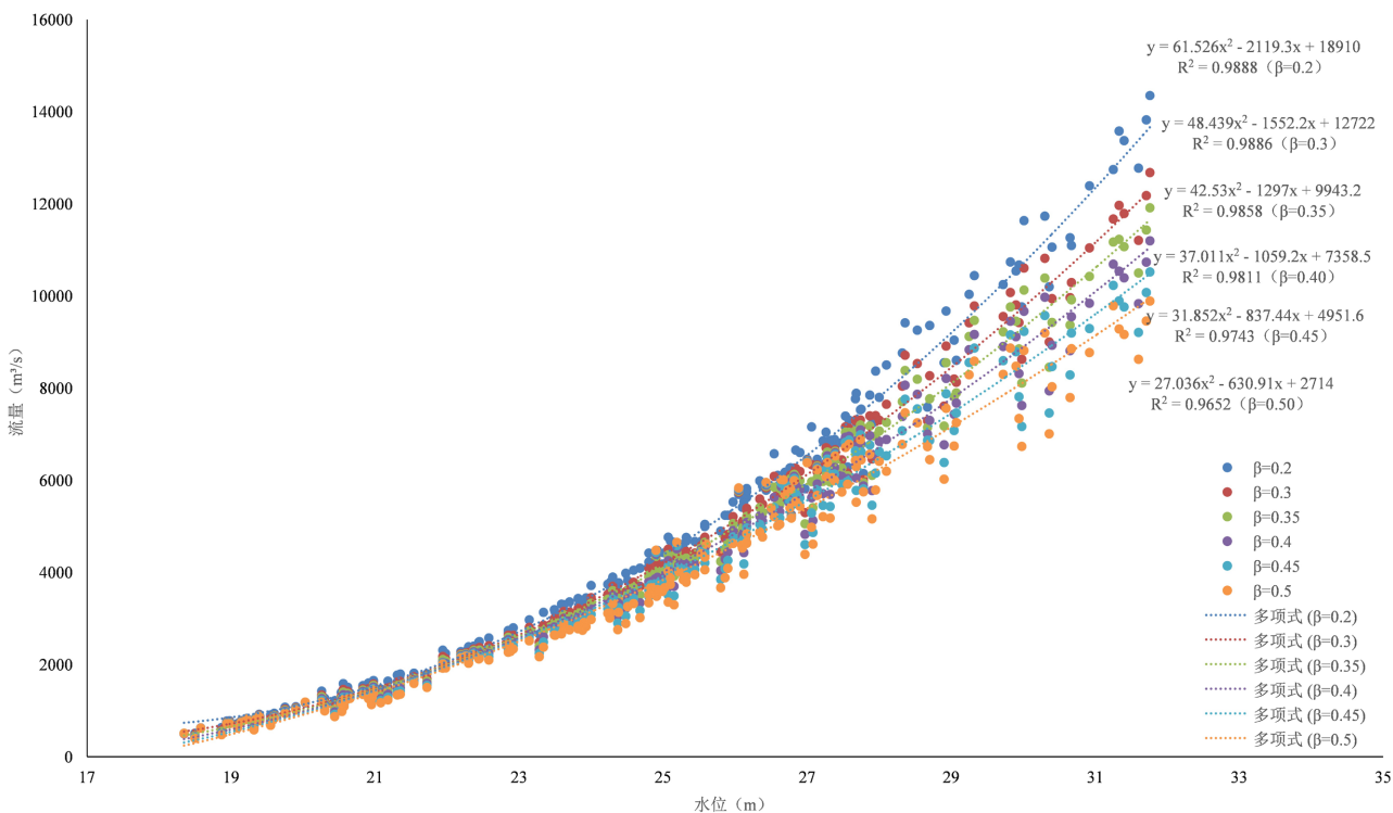
Figure 3. Correlation analysis diagram of flow with drop \geq 0.7 m
