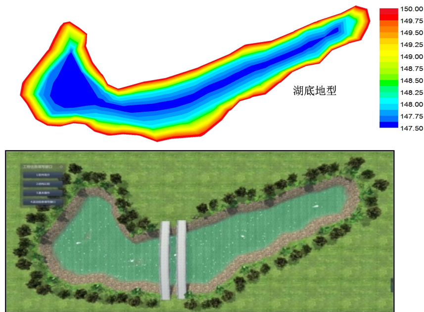
Figure 2. Model of aquatic ecological environment created with Unity3D 图 2. 利用 Unity3D 创建的水生态环境模型
