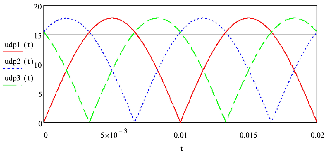
Figure 9. Open circuit voltage in three states after voltage division
