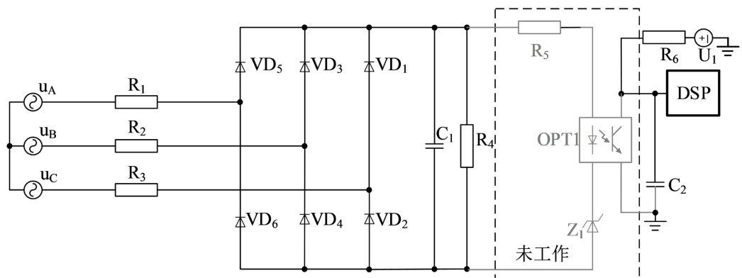
Figure 2. Normal pressure working state
