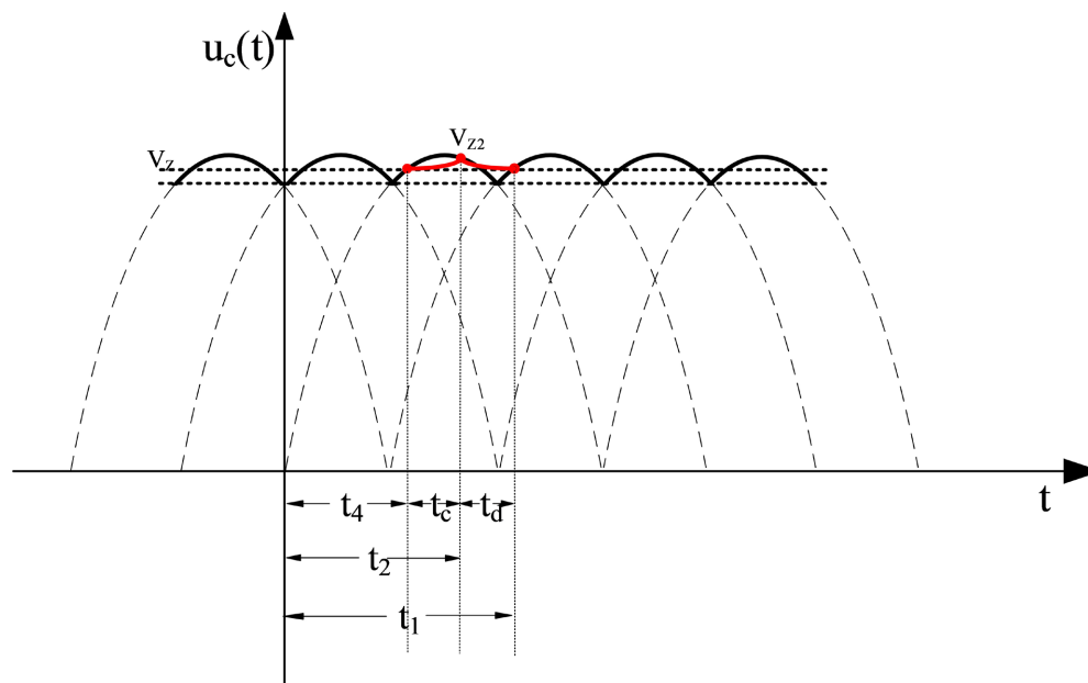
Figure 10. Waveform diagram of charging voltage of bridge arm capacitor and actual voltage of bridge arm capacitor
