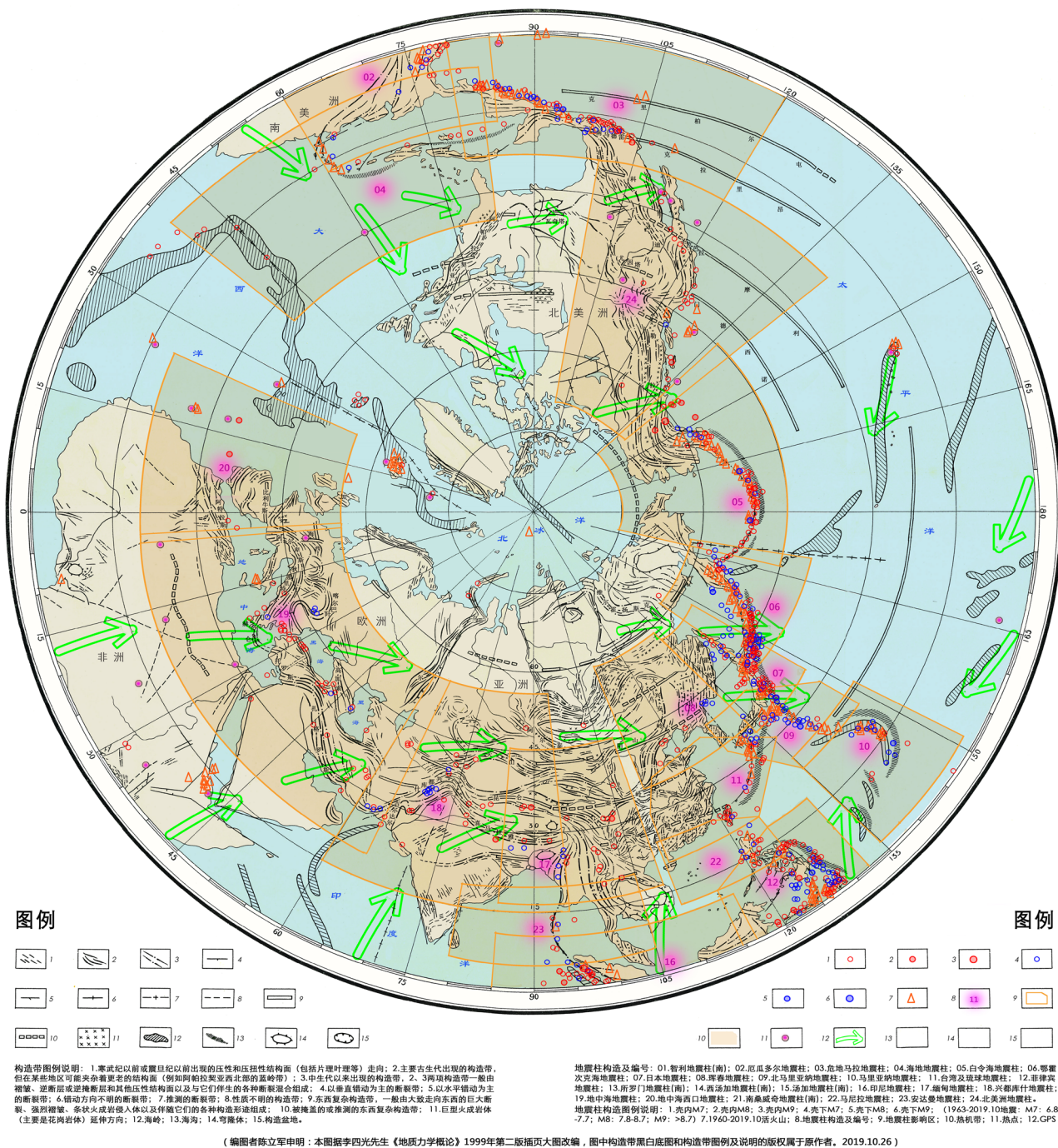
Figure 3. Simplified map of major tectonic belts exposed on the surface and seismic cone tectonics in the upper mantle of the Northern Hemisphere (adaptation from Li si Guang's "Geomechanics", 2nd edition, 1999, p. 136)
