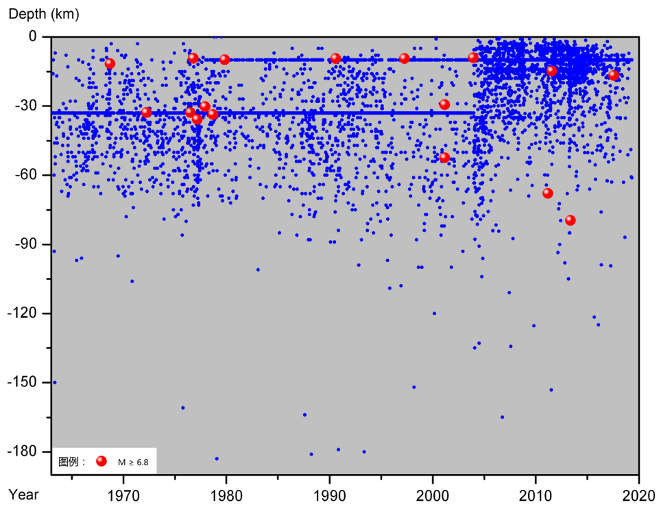
Figure 7. The source depth sequence of the Iranian branch of the Seismic Cone Tectonic No.19-3 from ANSS earthquake catalogue (1963-2019.5, M \geq 4.0 ) 图 7. 伊朗地震柱分支依据 ANSS 地震目录的震源深度时序图(1963~2019.5, M \geq 4.0 )
