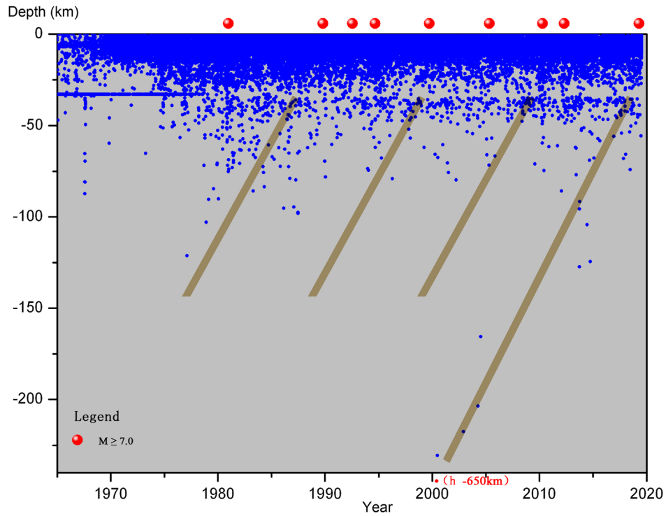
Figure 6. The focal depth sequence diagram of U02 Mini Seismic Cone Tectonic, USA (1965-2019.7, intracrustal earthquake M3.0+, subcrustal earthquake M2.0+) 图 6. 美国 U02 地震子柱构造的震源深度时序图(1965~2019.7, 壳内地震 M \geq 3.0 , 壳下地震 M \geq 2.0 )
