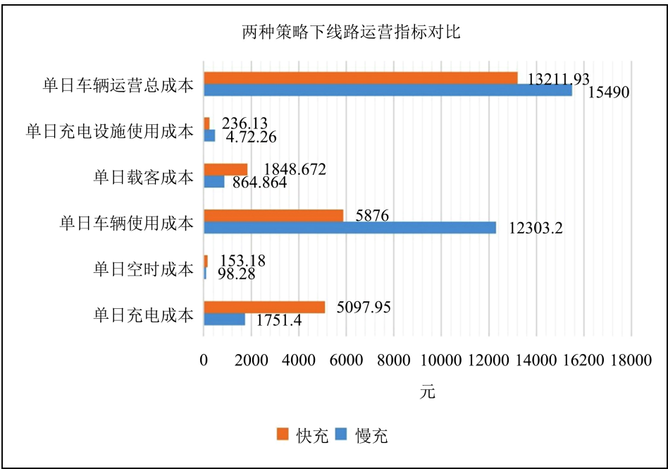
Figure 3. Comparison of line operation indicators under two strategies 图 3. 两种策略下线路运营指标对比
