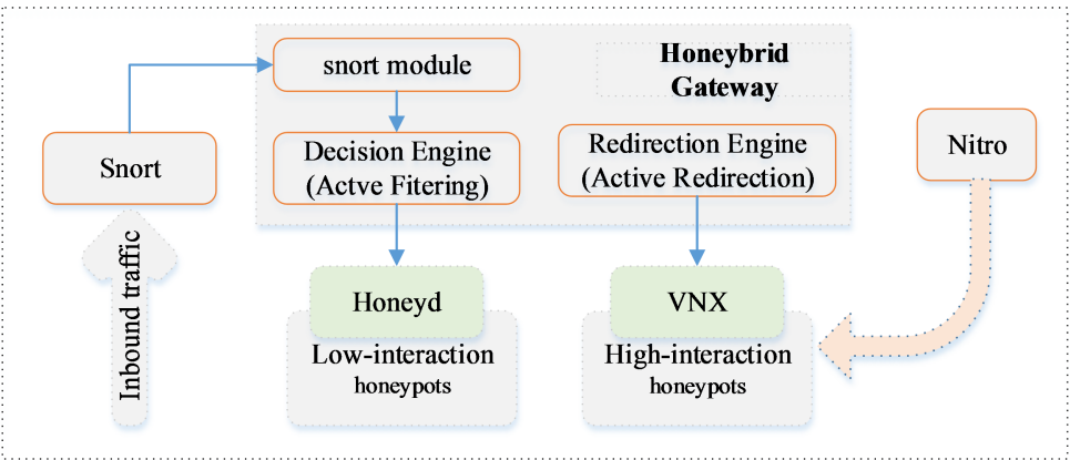
Figure 1. Scheme of snort and honeybrid 图 1. Snort 和 honeybrid 联合方案
