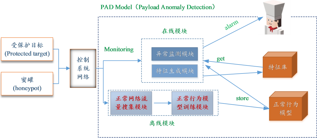
Figure 5. System architecture 图 5. 系统架构
