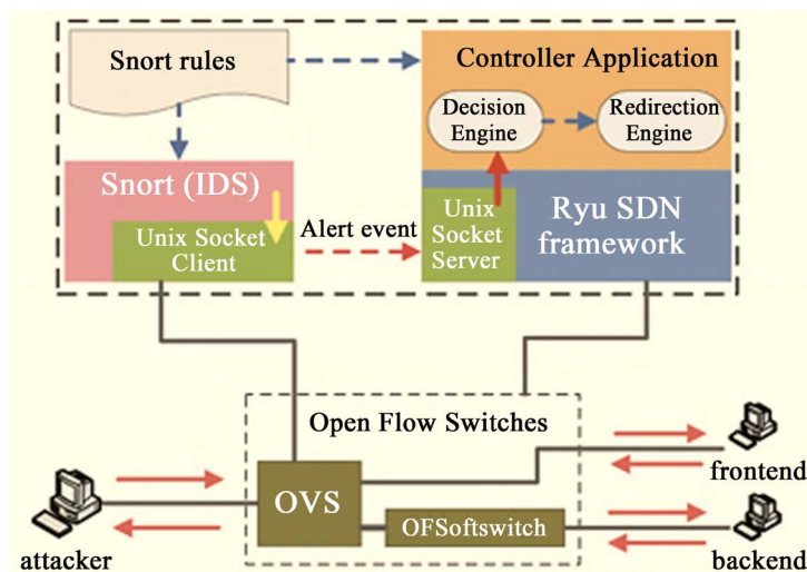
Figure 3. Mix frame work of Snort and SDN
