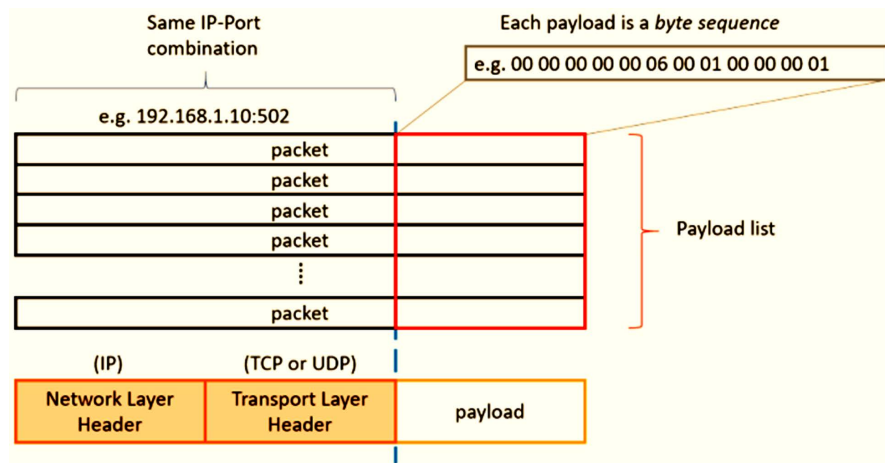
Figure 6. Normal network traffic
