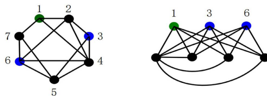
Figure 4. K_{4,3}^4 is P_0 -minor-free
