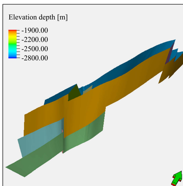
Figure 1. Three-dimensional fault model of upper Es3 in Wen 38 fault block 图 1. 文 38 断块沙三上亚段三维断层模型
