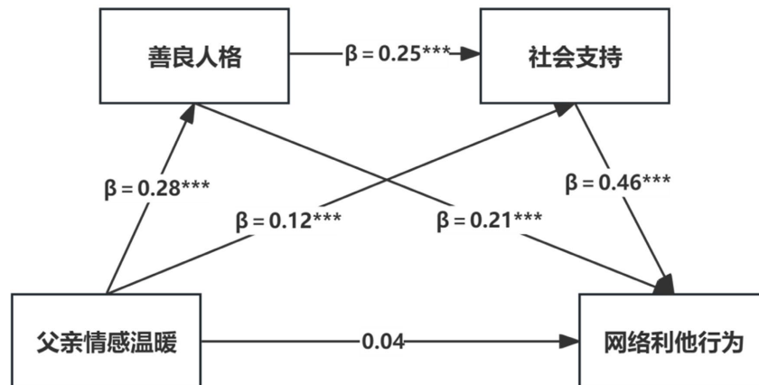
Figure 1. Path coefficient diagram of the model linking father's emotional warmth, benevolent personality, social support, and online altruistic behavior
