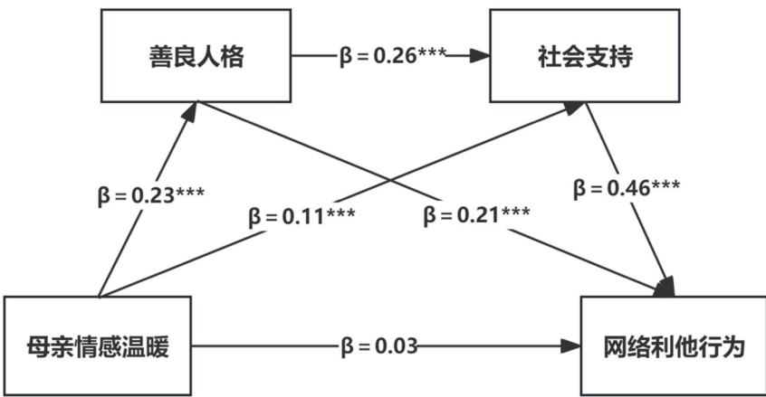
Figure 2. Path coefficient diagram of the model linking maternal emotional warmth, benevolent personality, social support, and online altruistic behavior
