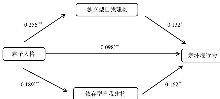
Figure 2. Path diagram of mediating effects
