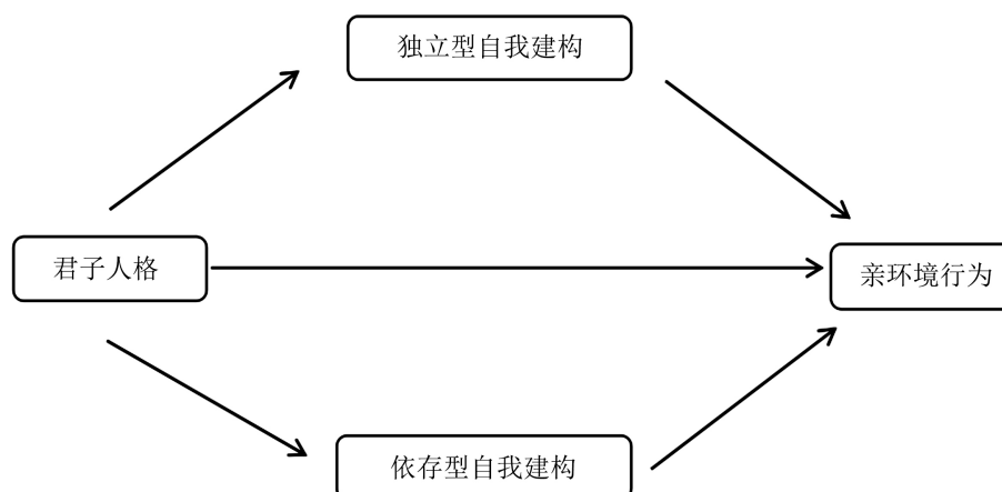
Figure 1. Model diagram between variables
