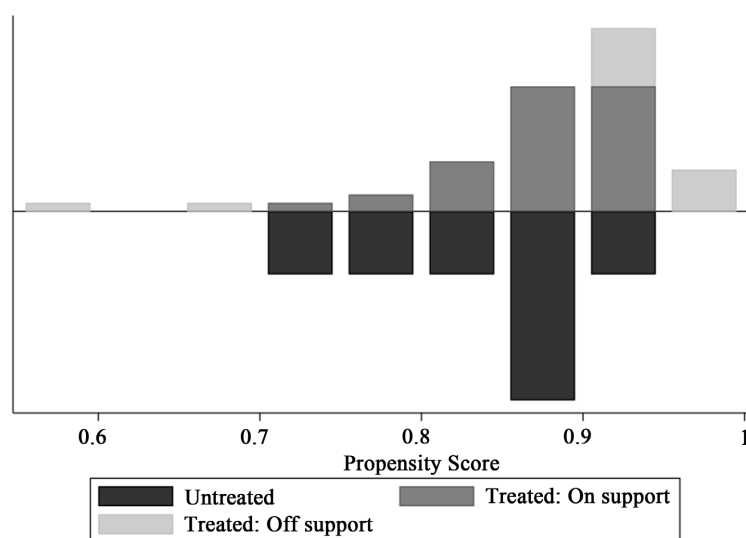
Figure 1. Propensity score matching plot
