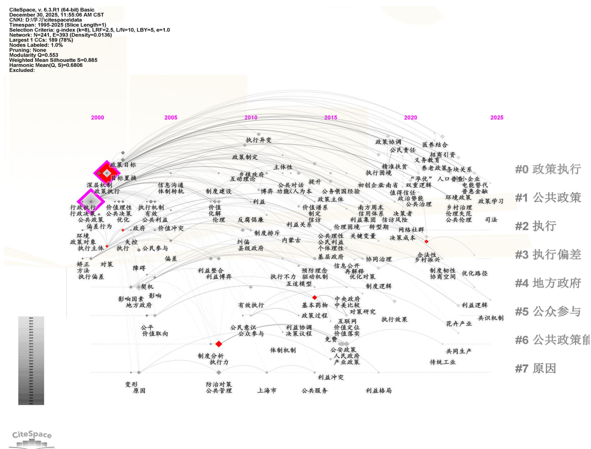
Figure 6. Development timeline graph of public policy implementation research
