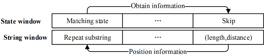
Figure 4. Diagram of compress matching 图 4. 压缩匹配原理示意
