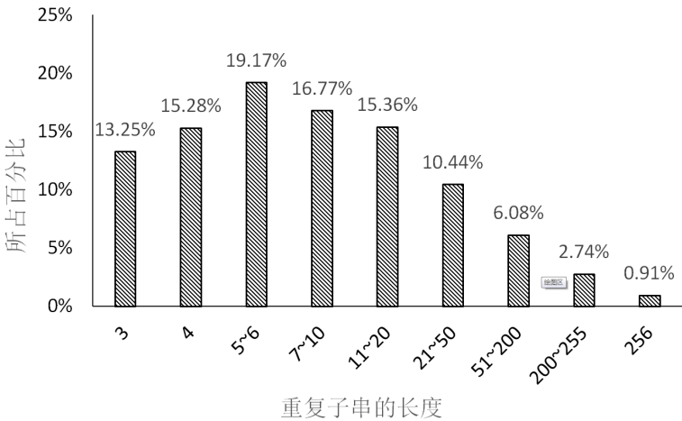
Figure 3. Length distribution of replicated sub-string in LZ77 图 3. LZ77 数据中重复子串的长度分布
