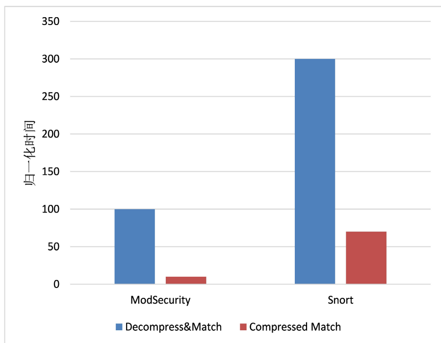
Figure 7. Normalize time
