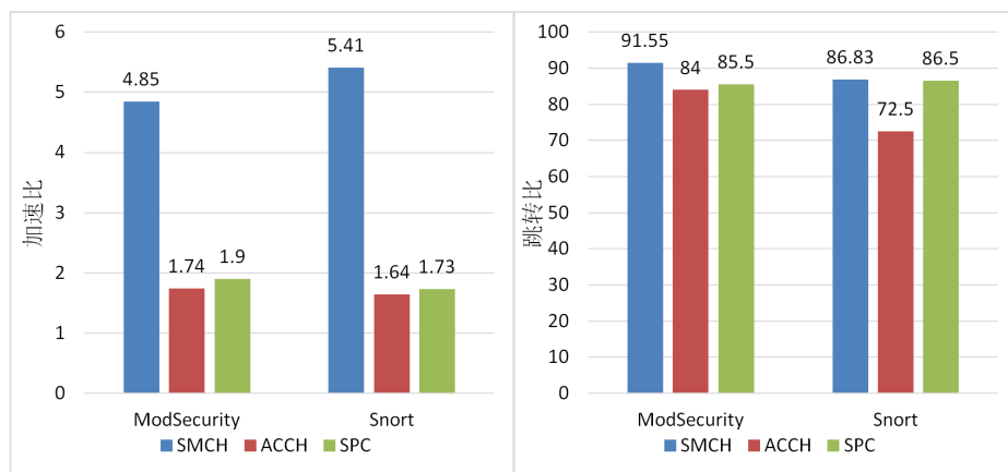
Figure 8. Accelerate rate &amp; skip rate
