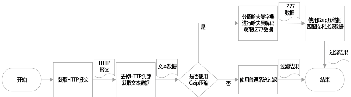
Figure 2. Filter procedure of compressed HTTP data 图 2. HTTP 压缩流量过滤流程
