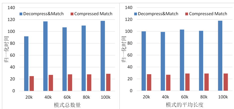
Figure 9. Normalize time when k = 1000
