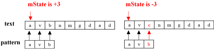
Figure 5. Illustration of mState 图 5. 匹配状态 mState 举例
