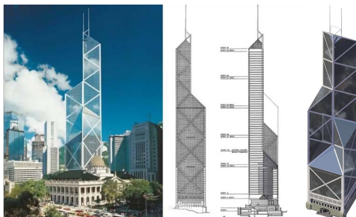
Figure 1. Geometric design of the building structure of the Bank of China Tower, Hong Kong 图 1. 香港中银大厦建筑结构的几何设计 ①
