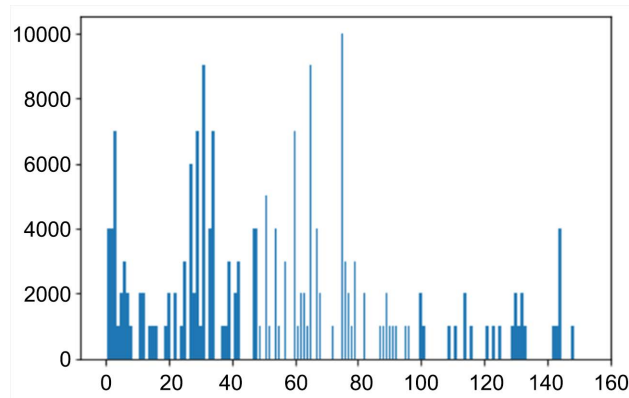
Figure 6. LightGBM indicator importance histogram 图 6. LightGBM 指标重要性柱状图
