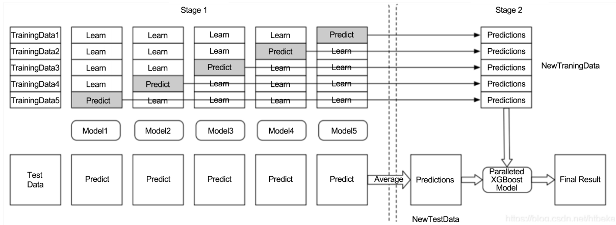
Figure 8. Stacking flowchart 图 8. Stacking 流程图
