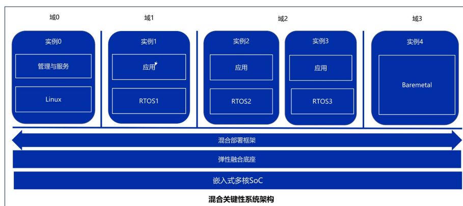
Figure 2. Mixed critical system architecture based on openEuler Embedded 图 2. 基于 openEuler Embedded 混合关键性系统架构
