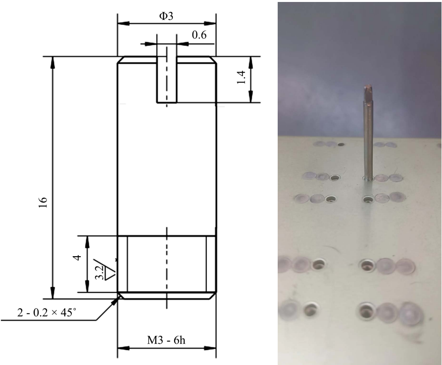
Figure 2. Concentric locating pin 图 2. 同心定位销钉
