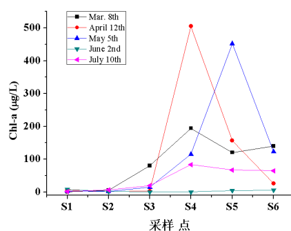
Figure 6. The concentration of chlorophyll a for each sample site 图 6. 各采样点 Chl-a 浓度
