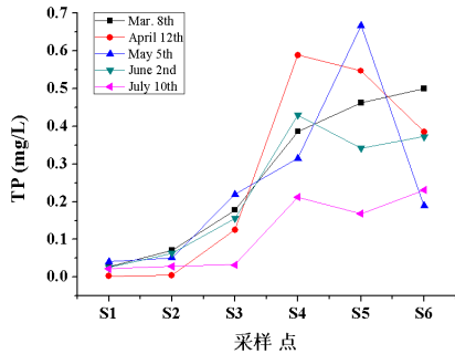
Figure 3. The concentration of total phosphorus for each sample site 图 3. 各采样点 TP 浓度
