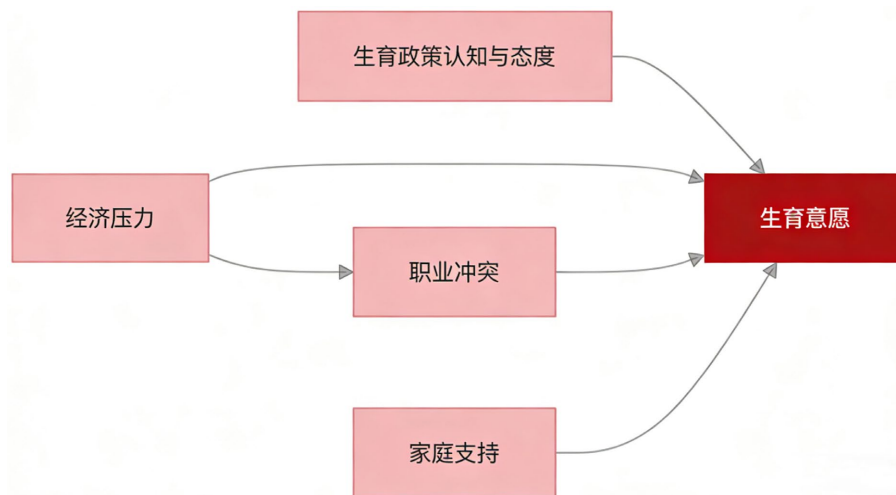
Figure 4. Path diagram of structural equation model
